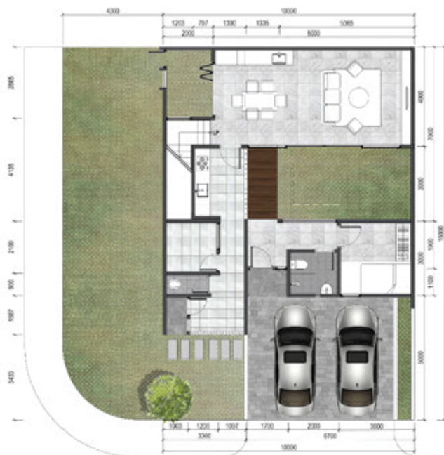
Lantai 1
